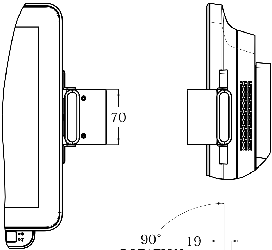
Option 1D BAR CODE SCANNER, P/N E267080
