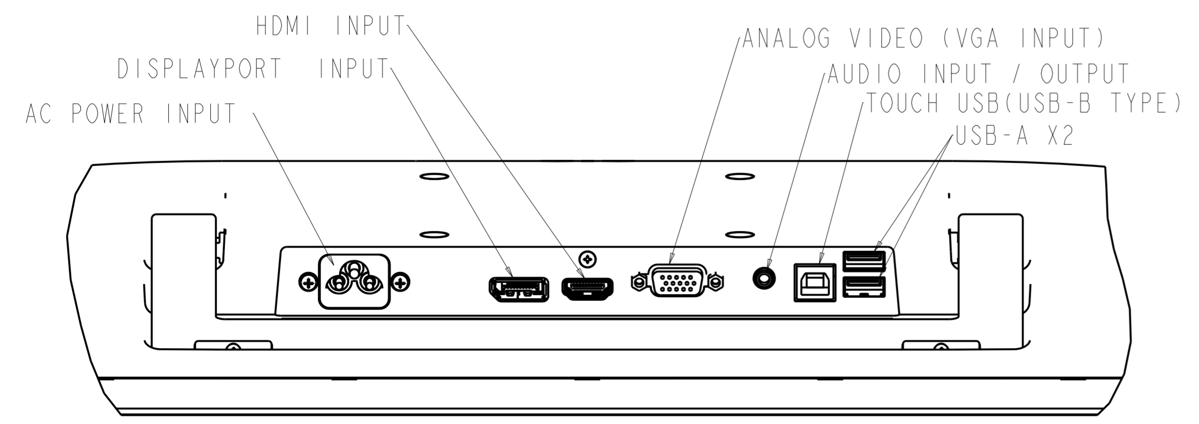
CONNECTOR PANEL
