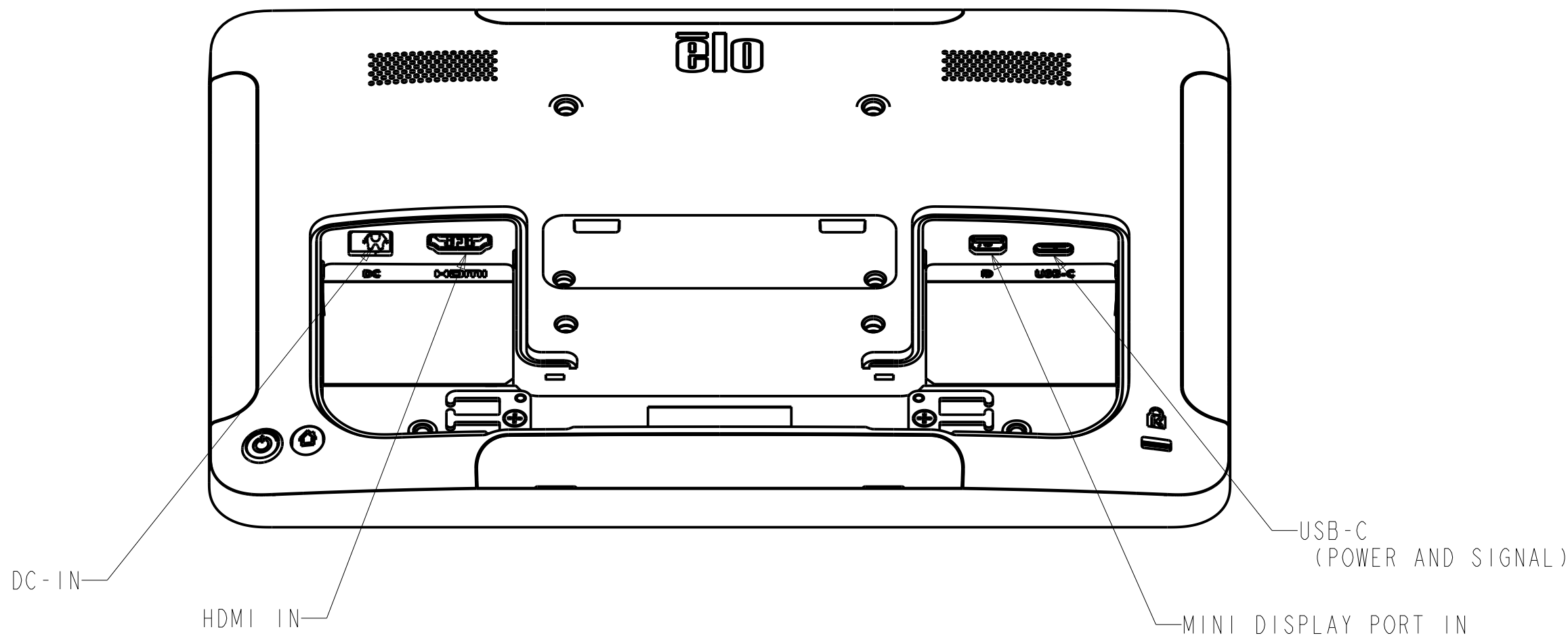
VIEW WITHOUT CABLE COVERS
